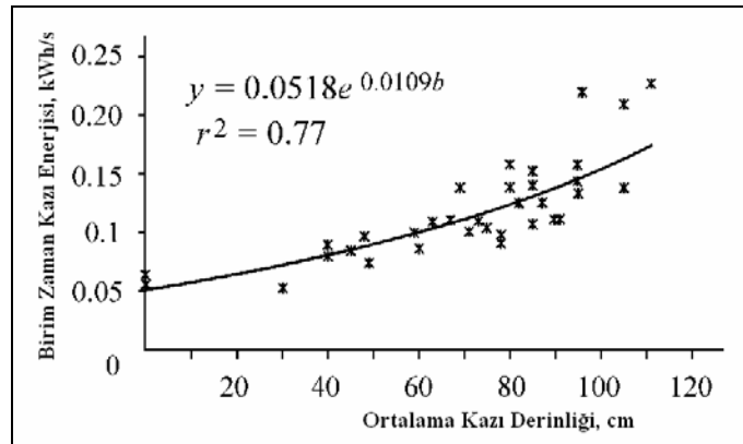
Figure 1. Depth-energy relationship.
